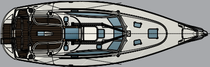
Decklayout
